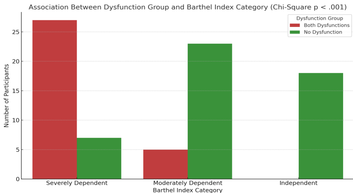
Figure 2: Chi Square Association of variables N=80
